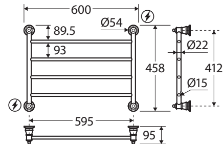
⚡ Wiring Positions
